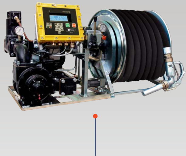
Measuring system for delivery trucks with ME3000 electronic register, hydraulic driven pump and hose reel winding, pneumatic VN valves, hose reel, PT-100 temperature probe (optional) hose and nozzle.
